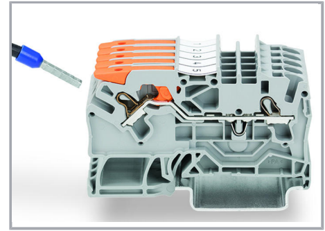
Push-in termination of fine-stranded conductors with ferrules
